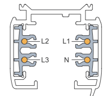
4 Wires | 3 Phases
