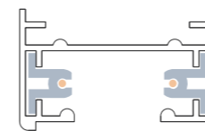
2 Wires | 1 Phase
