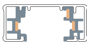
3 Wires | 1 Phase
