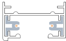
2 Wires | 1 Phase
