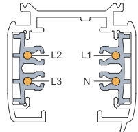
4 Wires | 3 Phases
